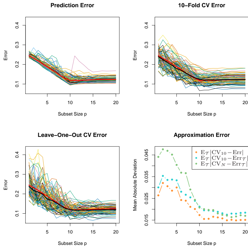
FIGURE 7.14. Conditional prediction-error Err_{\mathcal{T}} , 10-fold cross-validation, and leave-one-out cross-validation curves for a 100 simulations from the top-right panel in Figure 7.3. The thick red curve is the expected prediction error Err , while the thick black curves are the expected CV curves E_{\mathcal{T}}CV_{10} and E_{\mathcal{T}}CV_N . The lower-right panel shows the mean absolute deviation of the CV curves from the conditional error, E_{\mathcal{T}}|CV_K - Err_{\mathcal{T}}| for K = 10 (blue) and K = N (green), as well as from the expected error E_{\mathcal{T}}|CV_{10} - Err| (orange).
