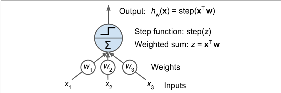
Figure 10-4. Threshold logic unit
