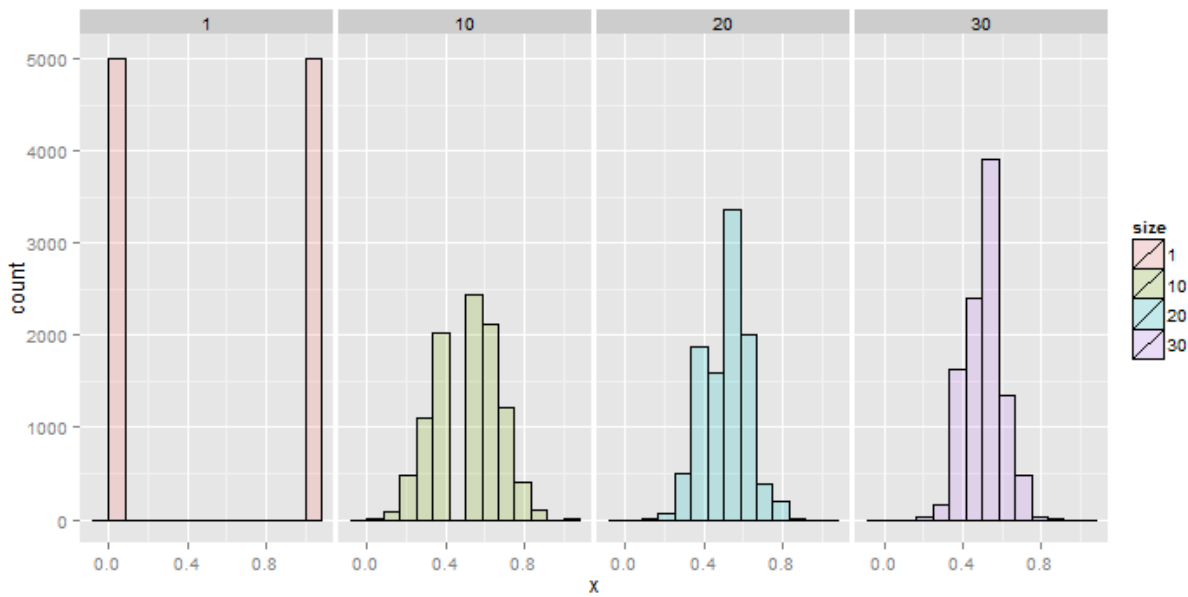
Simulation of coin flips
