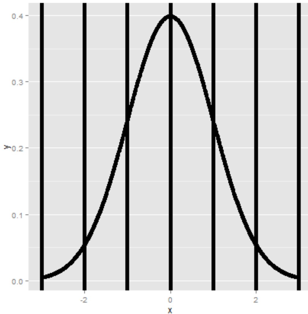
Standard normal reference lines.
