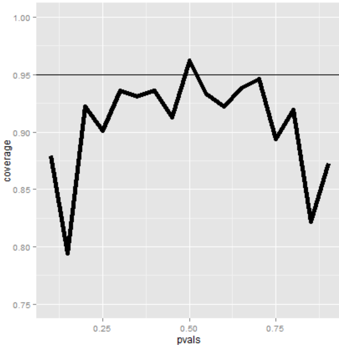
Plot of Wald interval coverage.
