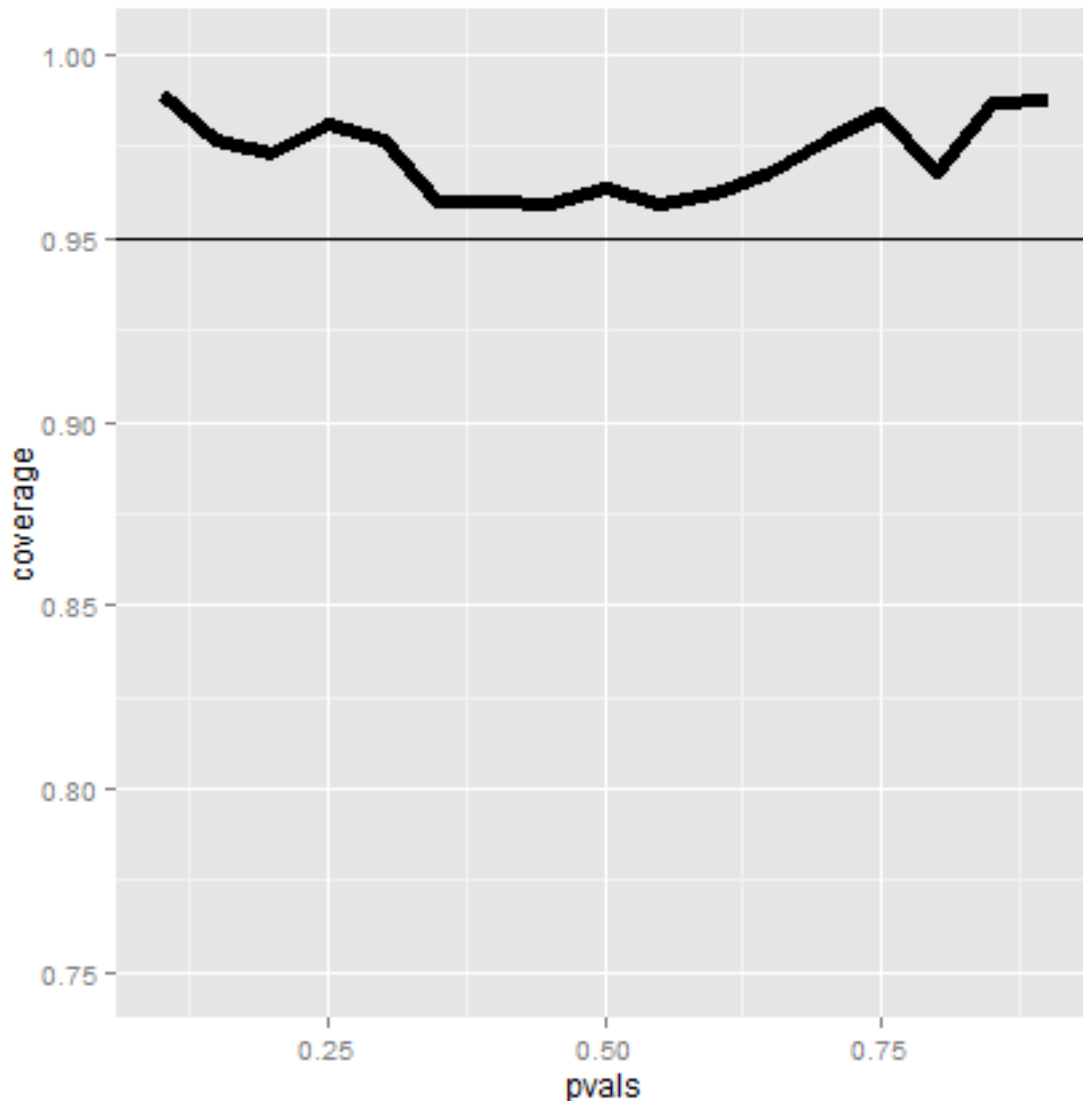
Coverage of the Agresti/Coull interval with n = 20
