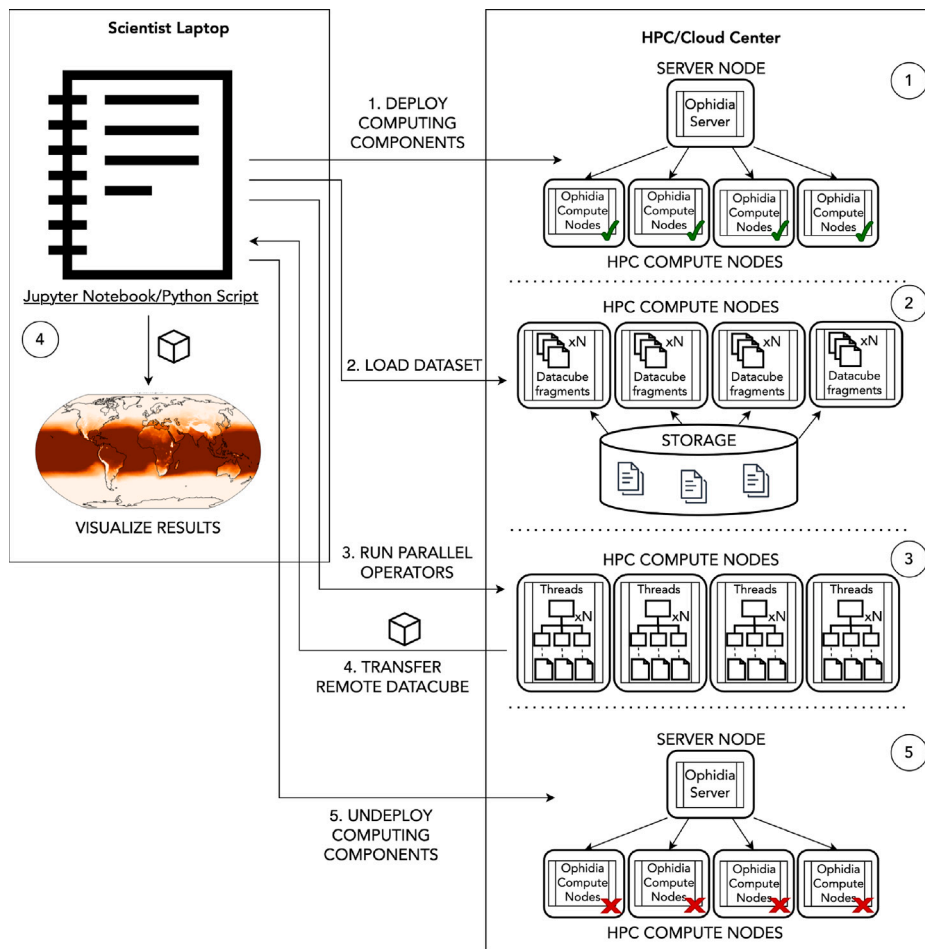
Fig. 2. Main steps in a HPDA application implemented with PyOphidia for running remote parallel processing on a HPC infrastructure [WITH COLORS].
